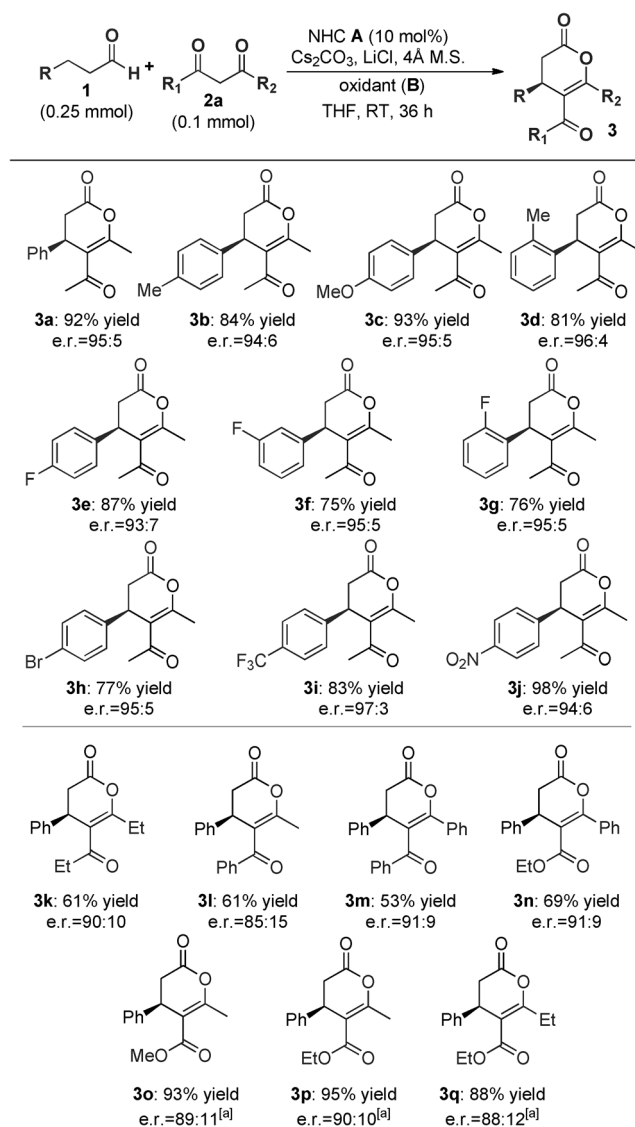
Scheme 2. Scope of the reaction. Reaction conditions: 1 (0.25 mmol), 2 (0.1 mmol), A (0.01 mmol), B (0.4 mmol), 4 Å M.S. powder, THF (1 mL), 36 h. Yields of isolated products based on 2a . Enantiomeric ratio of 3a , determined by HPLC on a chiral stationary phase. [a] Reactions performed without LiCl. When LiCl was used as an additive, the desired product was not obtained.
