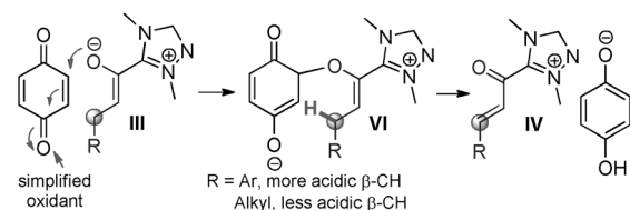
Scheme 3. Proposed pathways for key oxidation steps.
