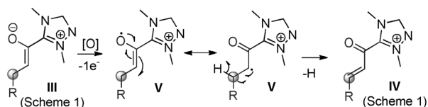
a) single-electron-transfer (radical) mechanism:
