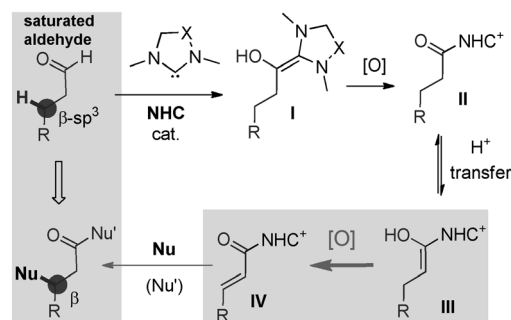
Scheme 1. Direct \beta -functionalization of saturated aldehydes: a working hypothesis.
