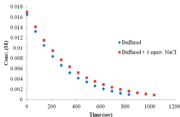
Figure 11. Plot comparing two 0.02 M 1 vs time in 60% D 2 O/acetone- d 6 . Buffered vs buffered + 3 equiv NaCl.
