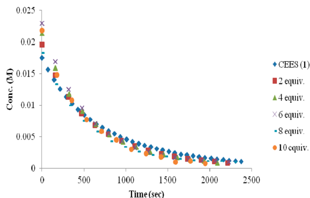
Figure 15. Plot showing 0.02 M 1 vs time in 60% \text{D}_2\text{O} /acetone- d_6 with increasing amounts of 2 .
