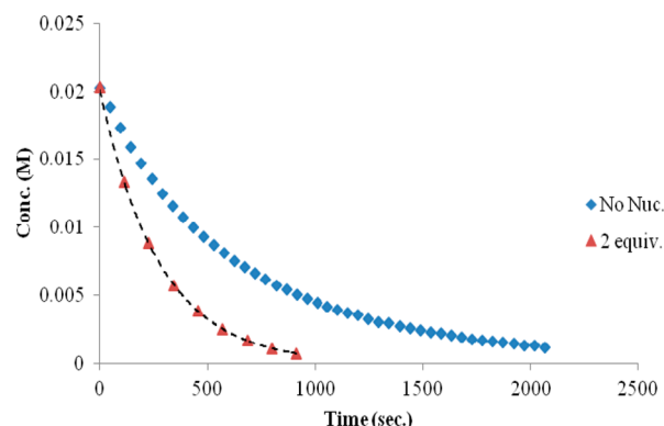
Figure 13. Plot showing 0.02 M 1 vs time in 60% D 2 O/acetone- d 6 with 2 equiv of sodium thiosulfate. The dashed line shows the first-order fit ( f(x) = ae^{bx} ).
