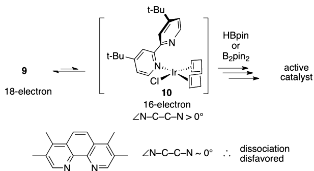
Scheme 4. Accessibility of κ 1 -Intermediates for Dipyrilidyl and Phenanthroline Ligands
