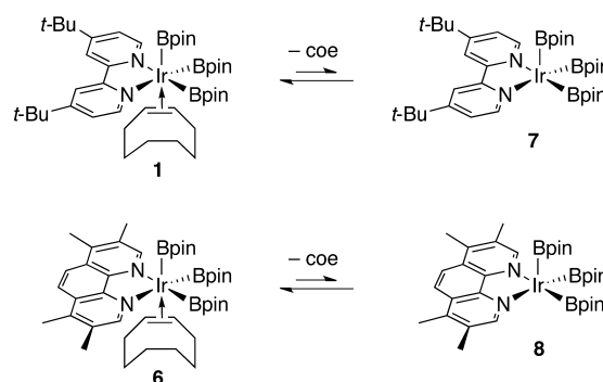
Scheme 2. Isolable Precatalysts and Equilibria Generating Active Intermediates
