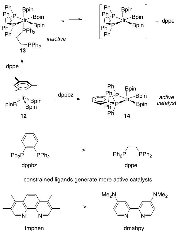
Scheme 5. Effects of Ligand Geometries on Catalysis
