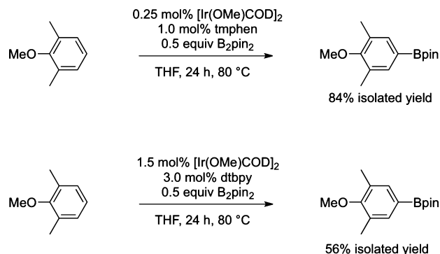
Scheme 7. Low Loading Borylation of an Electron-Rich Substrate
