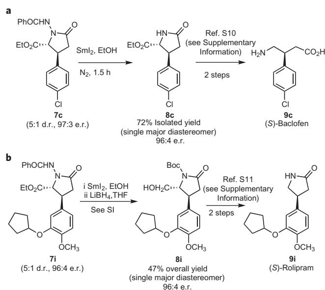
Figure 2 | Synthetic transformation to bioactive molecules. a , Preparation of drug ( S )-Baclofen ( 9c ) from lactam 7c . b , Lactam 7i could be converted to ( S )-Rolipram ( 9i ), which is a potent inhibitor for the treatment of central nervous disorders.
