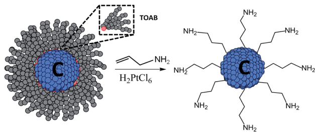
Scheme 1 Chemical passivation and functionalisation of the CQDs using a platinum-catalysed concerted reaction. CQDs are synthesized by reduction of \text{CCl}_4 within TOAB reverse micelles in toluene.
