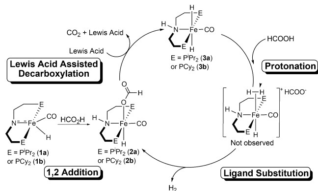
Scheme 2. Proposed Mechanism of FA Dehydrogenation
