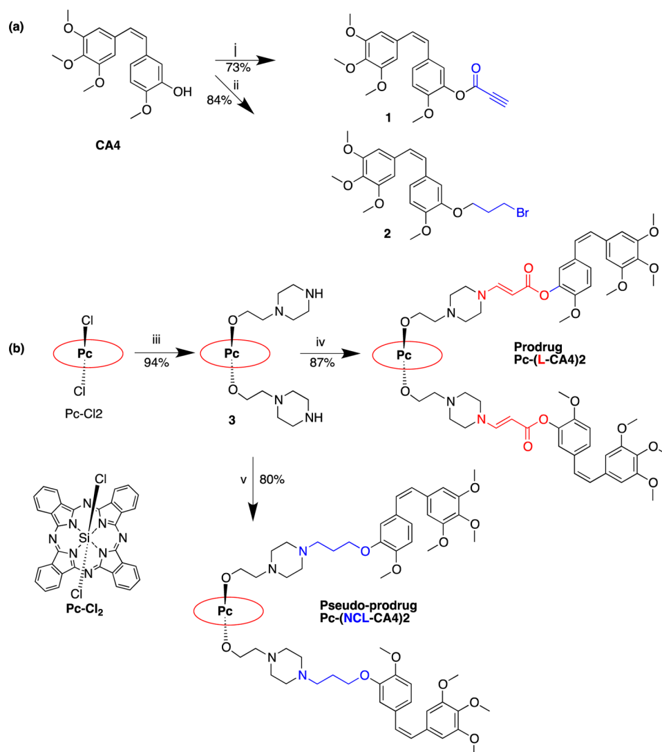
Scheme 1. Synthesis of \text{Pc}-(\text{L-CA4})_2 and \text{Pc}-(\text{NCL-CA4})_2 a
