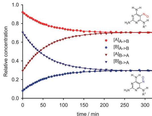
Fig. 5 Interconversion of rotamers 1A and 1B . Interconversion was monitored by ^1\text{H} NMR spectroscopy in a \text{DMSO}-d_6 solution. \text{R}^1 = \text{CH}_2\text{--CH}_2\text{--O--CH}_2\text{--P(O)(OEt)}_2 .
