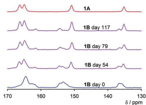
Fig. 3 The aromatic region of 13 C CP-MAS solid-state NMR spectra of planar rotamers 1A and 1B . Solid amorphous 1B slowly transforms into solid crystalline 1A . The full spectrum is available in Fig. S1 in ESI†.
