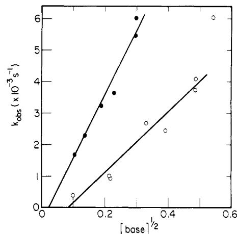
Figure 2. Graph of the pseudo-first-order rate constant, k_{\text{obsd}} , vs. [\text{base}]^{1/2} for reaction with \text{Mn}(\text{CO})_5(\text{CH}_3\text{CN})^+ in \text{CH}_3\text{NO}_2 at 31.8 °C: \circ = pyridine; \bullet = 4-methylpyridine.
