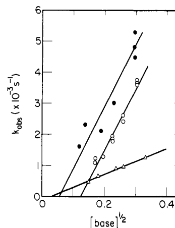
Figure 3. Graph of the pseudo-first-order rate constant, k_{\text{obsd}} , vs. [\text{base}]^{1/2} for reaction with \text{Mn}(\text{CO})_5(\text{CH}_3\text{CN})^+ in \text{CH}_3\text{NO}_2 at 31.8 °C: \circ = N -benzylimidazole; \bullet = 2-methylpyridine. \blacktriangle = reaction of \text{Mn}(\text{CO})_5\text{NC}_5\text{H}_5^+ with pyridine.
