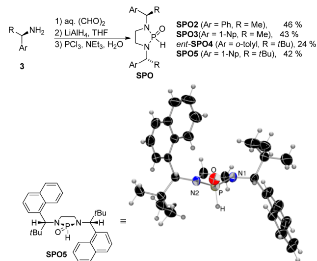
Scheme 2. Synthesis and X-Ray Crystal Structure of Diaminophosphine Oxide SPOs
