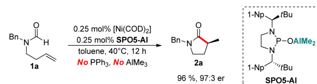
Scheme 5. Catalytic Performance of the Preformed Lewis Acid/Ligand SPO5-Al
