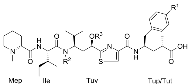
Figure 1. Chemical structures of natural tubulysins 1 . R 1 , R 2 , and R 3 : various substituents (see Table 1).
