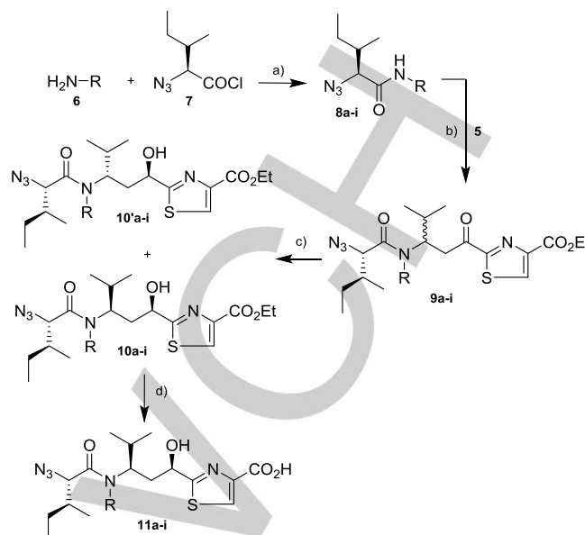
Scheme 2. Synthesis of the azido derivatives 8a-i . Reagents and conditions: (a) i -Pr 2 EtN, CH 2 Cl 2 , 0 °C, 1h, 80 to 99%; (b) KHMDS, anhydrous THF, -78 °C, 1h, overall 15 to 54%; (c) ( S )-CBS, anhydrous THF, BH 3 ·Me 2 S 10M, from 0 °C to rt, overall 32 to 81%; (d) LiOH, THF/H 2 O 4:1, 12h, rt, 60 to 99%
