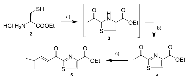
Scheme 1. Synthesis of the \alpha,\beta unsaturated thiazolyl ketone 5 . Reagents and conditions: (a) methylglyoxal, NaHCO 3 , EtOH-H 2 O (1:1), overnight; (b) MnO 2 , MeCN, 65 °C, overnight (52% over two steps); (c) isobutyraldehyde, TiCl 4 , Et 3 N, anhydrous THF, from -78 °C to rt (70%).
