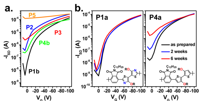
Figure 7. (a) Comparison of P1–P5-based OTFT transfer characteristics. (b) Comparison of transfer characteristics of BTzOR-based polymer P1a and BTOR-based P4a BGTC OTFTs stored and characterized in air.
