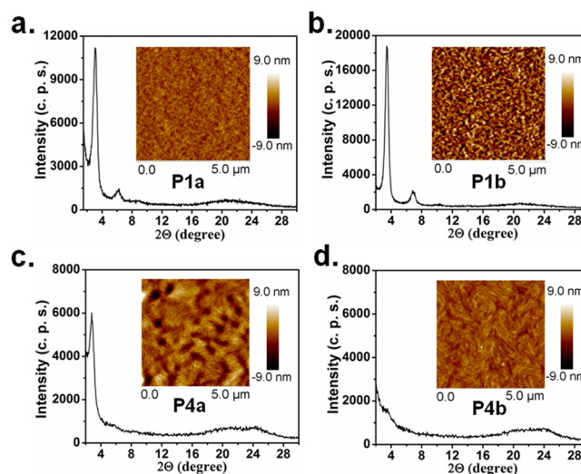
Figure 8. XRD scattering patterns and AFM data (inset: 5 \times 5 μm topographic images) of BTzOR-based polymer P1 and BTOR-based polymer P4 films fabricated under conditions that yield the best-performing thin-film transistors.
