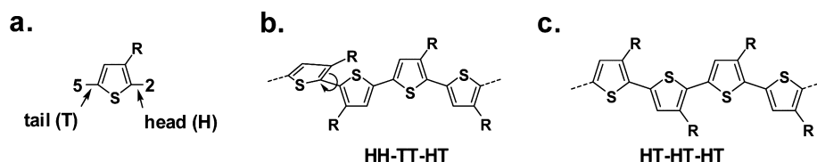
Figure 1. Chemical structures of (a) 3-alkylthiophene, in which the 2-position is designated head (H) and the 5-position is designated tail (T); (b) regioirregular poly(3-alkylthiophene), which contains head-to-head (HH), tail-to-tail (TT), and head-to-tail (HT) linkages; and (c) regioregular poly(3-alkylthiophene), which contains exclusively head-to-tail (HT) linkages.
