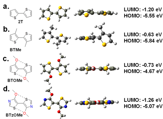
Figure 3. Chemical structures, optimized geometries, LUMO energies, and HOMO energies for (a) bithiophene ( 2T ), (b) 3,3'-dimethyl-2,2'-bithiophene ( BTMe ), (c) 3,3'-dimethoxy-2,2'-bithiophene ( BTOMe ), and (d) 4,4'-dimethoxy-5,5'-bithiazole ( BTzOMe ). Calculations were carried out at the DFT//B3LYP/6-31G** level.
