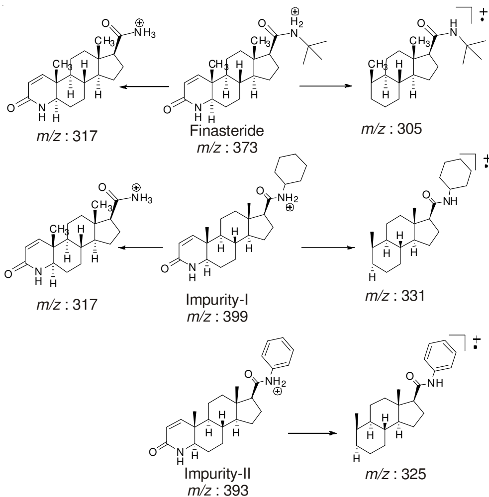
Fig. 9. Mass fragmentation of impurity-I and impurity II
