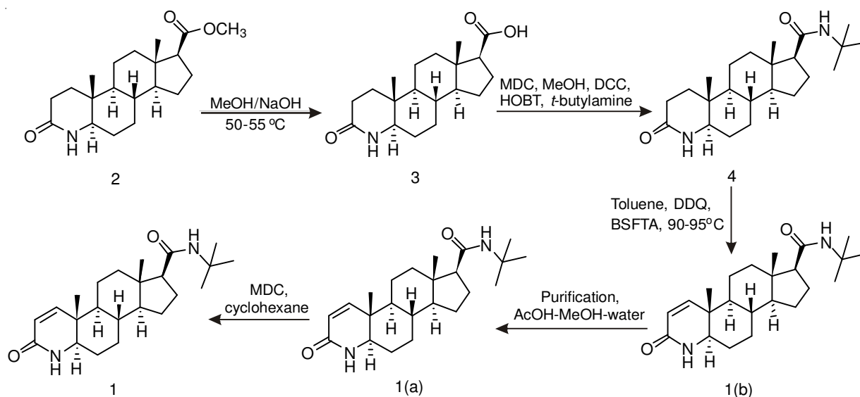
Scheme-I: Finasteride ( 1 ) manufacturing process 5
