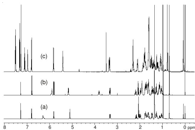
Fig. 6. Overlay of ^1\text{H} NMR data: (a) Finasteride, (b) impurity-I and (c) impurity-II
