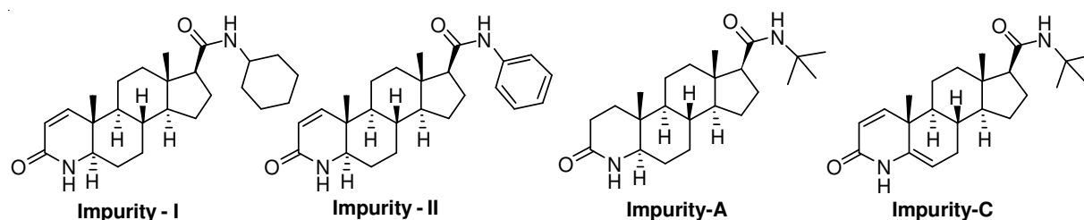
Fig. 2. Impurities of finasteride ( 1 )
