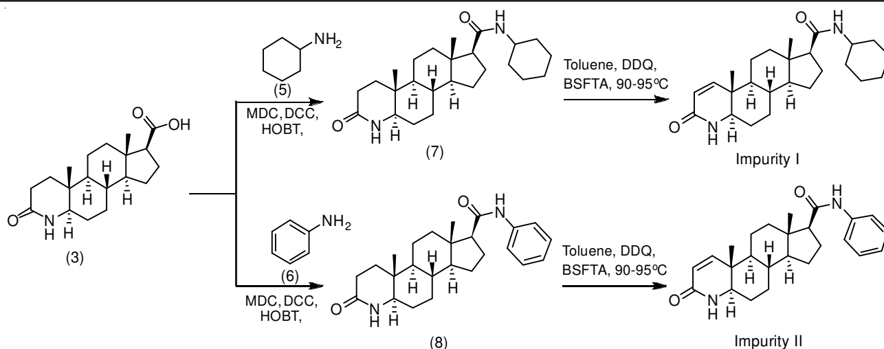
Scheme-II: Synthesis of Finasteride impurities
