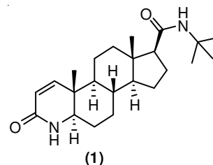
Fig. 1. Structure of finasteride
