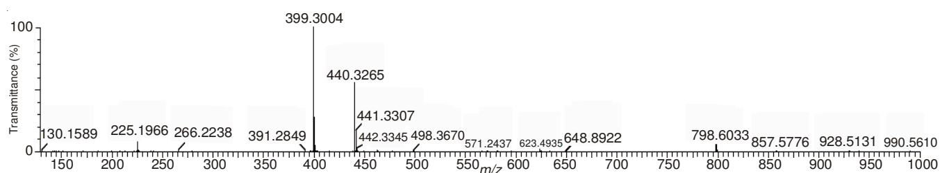
Fig. 5. MS/MS spectrum of Impurity-I
