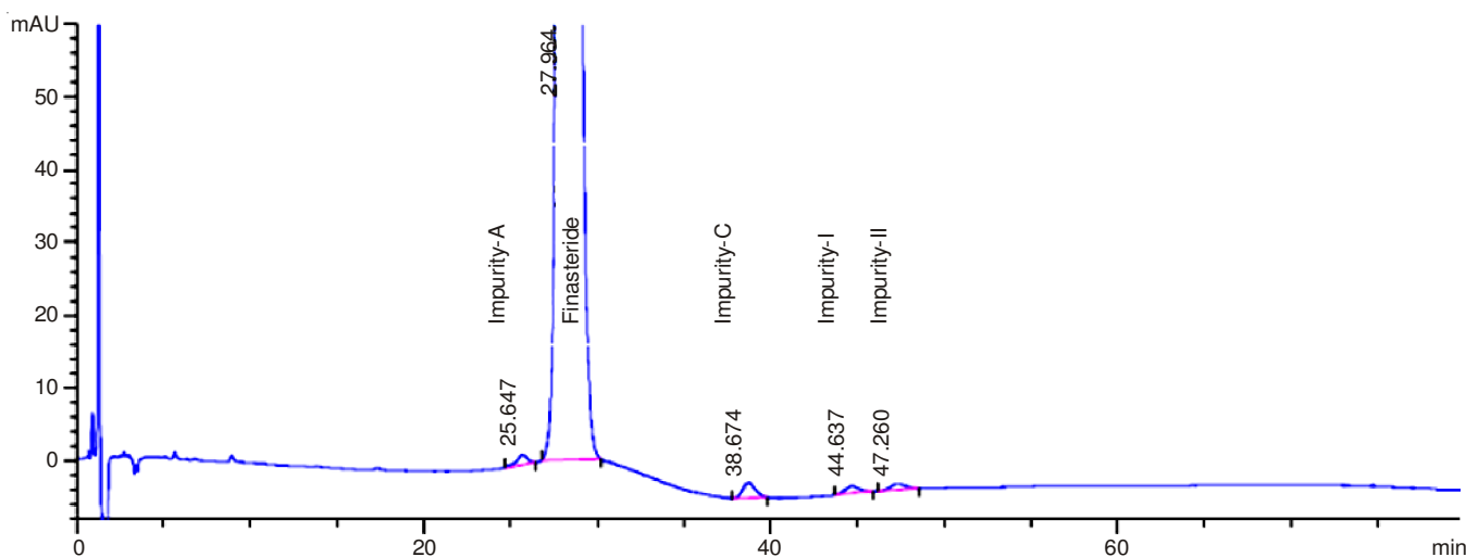
Fig. 3. HPLC chromatogram of crude Finasteride
