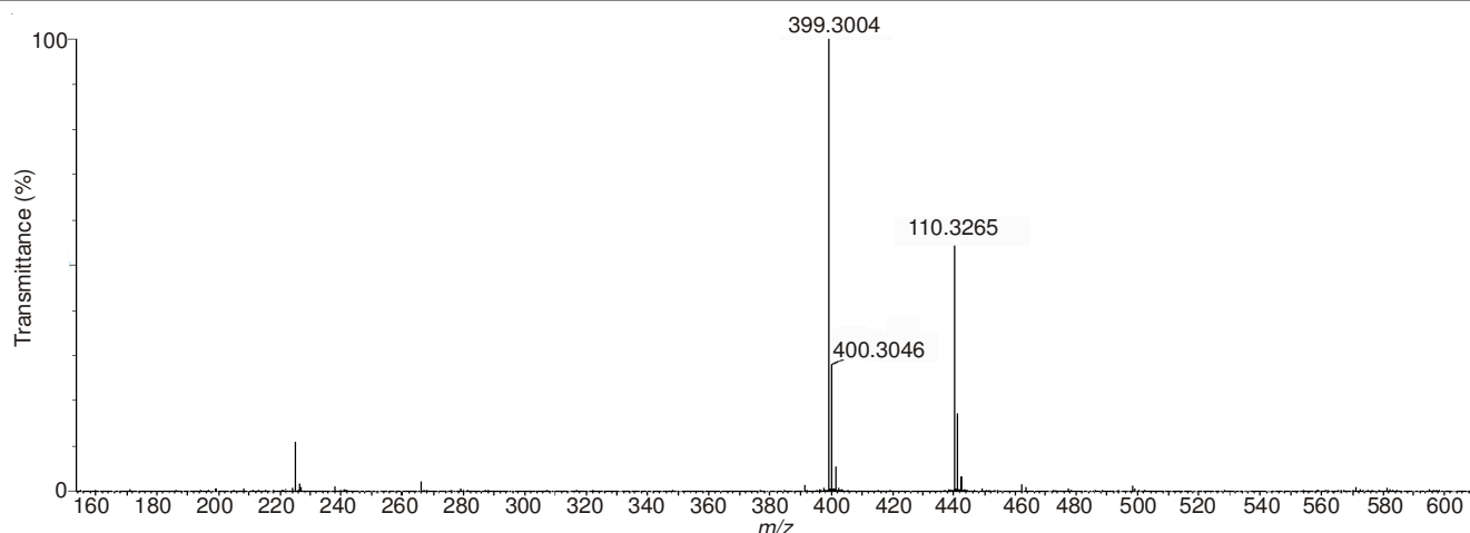
Fig. 4. UPLC-TOF mass spectrum of Impurity-I
