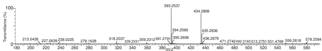
Fig. 8. MS/MS spectrum of Impurity-II
