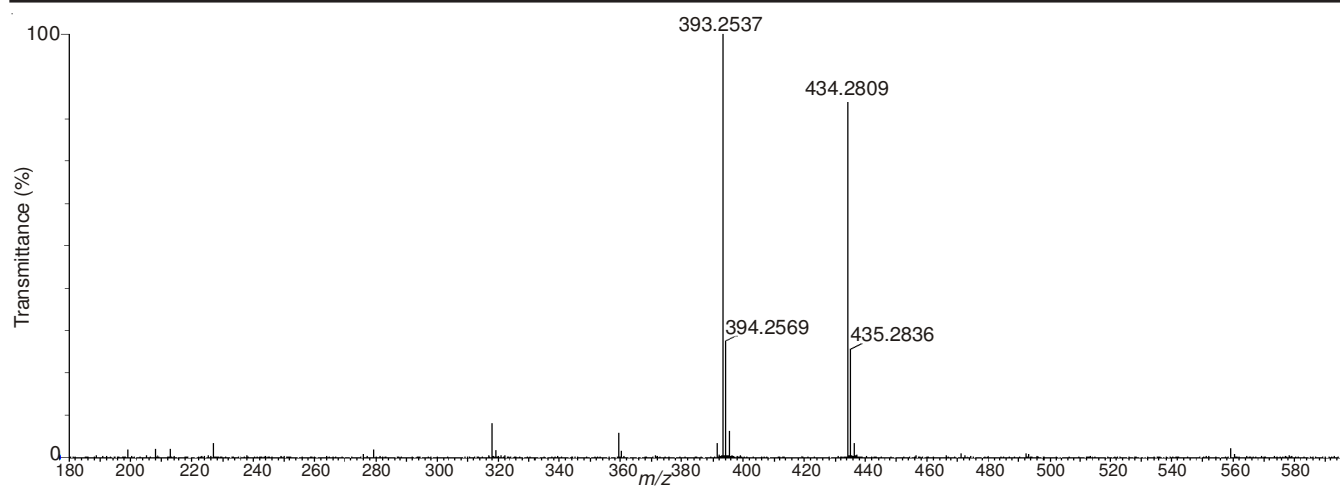
Fig. 7. UPLC-TOF mass spectrum of Impurity-II
