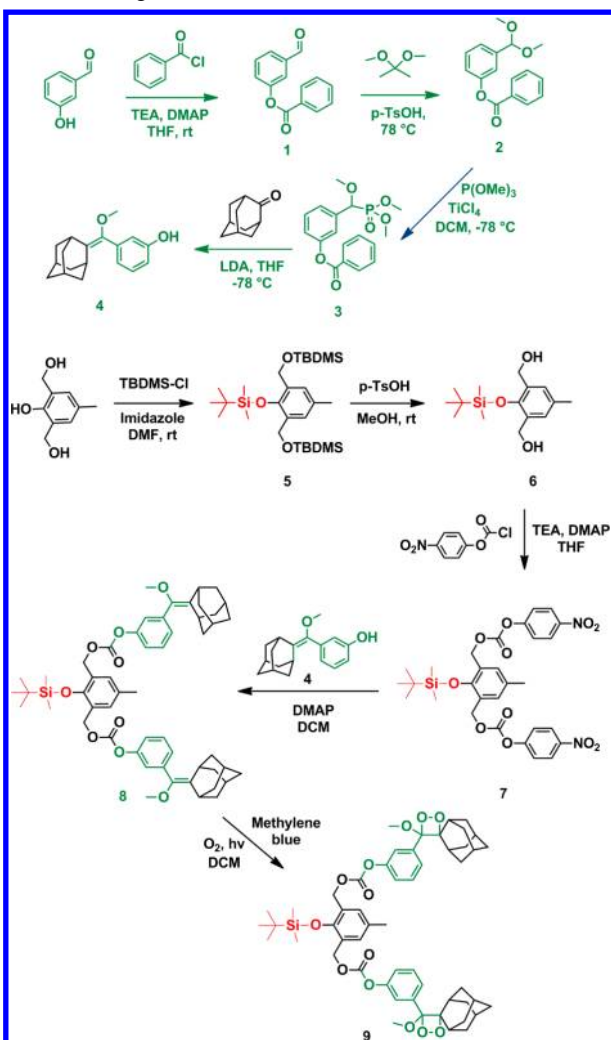
Scheme 1. Synthesis of the Self-Immolative Chemiluminogenic Fluoride Sensor
