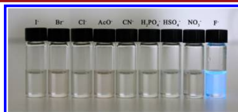
Figure 3. Selective chemiluminescent response of the fluoride probe 9 under ambient light.
