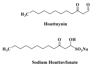
Fig. 1. The Chemical Structure of Houttuynin and Sodium Houttuynifonate
