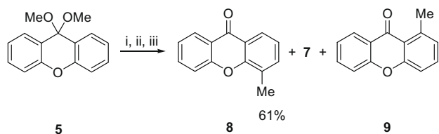
Scheme 2. Lithiation according to procedure B. 11 Reagents and conditions: (i) t -BuLi (1.5 equiv)/THP, –13 °C, 30 min; (ii) CH 3 I and (iii) H + /H 2 O.
