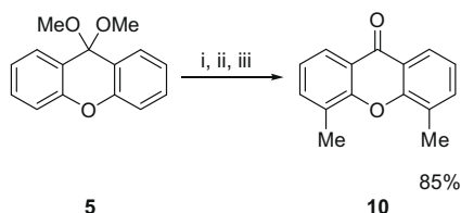
Scheme 3. Lithiation according to procedure C. 11 Reagents and conditions: (i) t -BuLi (3 equiv), t -BuOK (3 equiv)/THP, –13 °C, 30 min; (ii) CH 3 I and (iii) H + /H 2 O.
