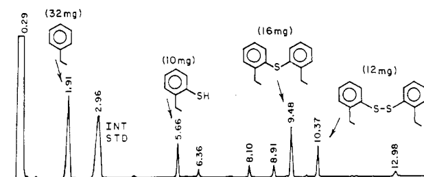
Figure 1. Gas chromatography trace of the volatiles formed in the hydrogenation of Fe 2 (C 8 H 6 S)(CO) 6 .
