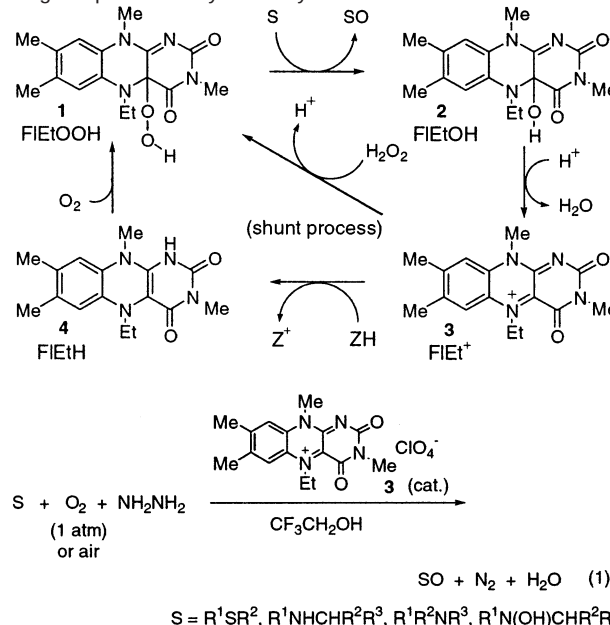
Scheme 1. Catalytic Cycle for the Oxidation of Flavoenzyme Using Simplified 5-Ethyl-3-methylumiflavin
