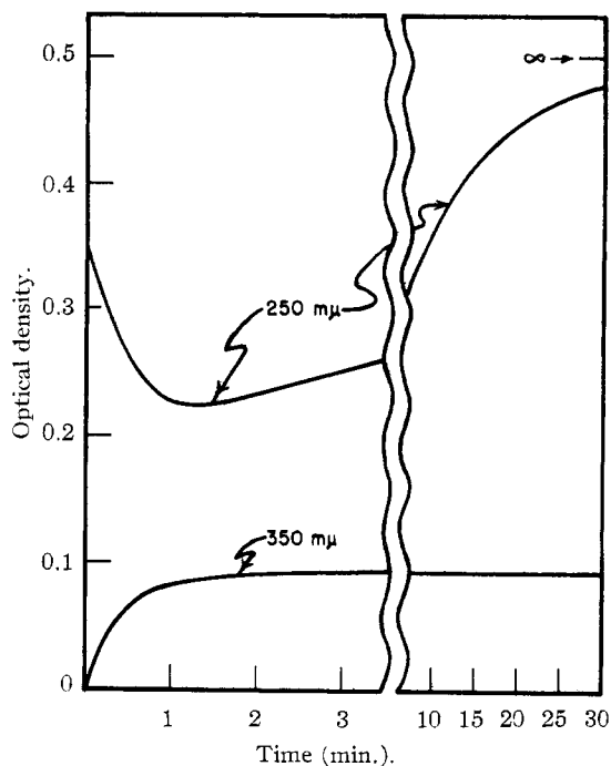
Fig. 1.—The \alpha -chymotrypsin-catalyzed hydrolysis of o -nitrophenyl cinnamate at pH 6.2 at 25° in phosphate buffers containing 10% acetonitrile. Measurements were taken on a Beckman DK-2 recording spectrophotometer: E = S \cong 0.42 \times 10^{-4} M .
