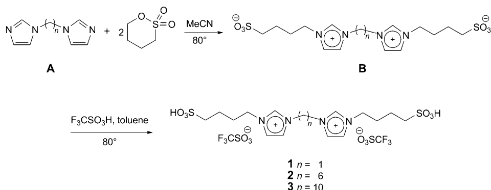
Scheme 1. Synthesis of the Novel Acidic Ionic Liquids 1–3
