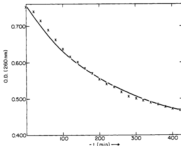
Figure 3. Plot of OD 260 vs. time for the methoxyaminolysis of 4,5-dihydro-3( H )-1,3-benzodiazepine (III), pH 7.11, 0.03 M K-phos, [CH 3 ONH 2 ] = 0.5 M ( T = 50 °C, \mu = 1.0, KCl). Solid line represents computer simulation curve to Scheme I. Onset of phase II at ca. 30 min; onset of phase III at ca. 5 h.
