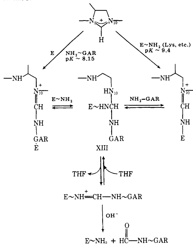
Scheme IV
