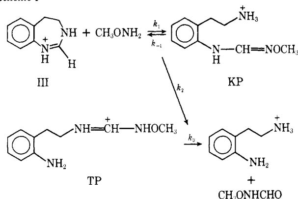
Scheme I
