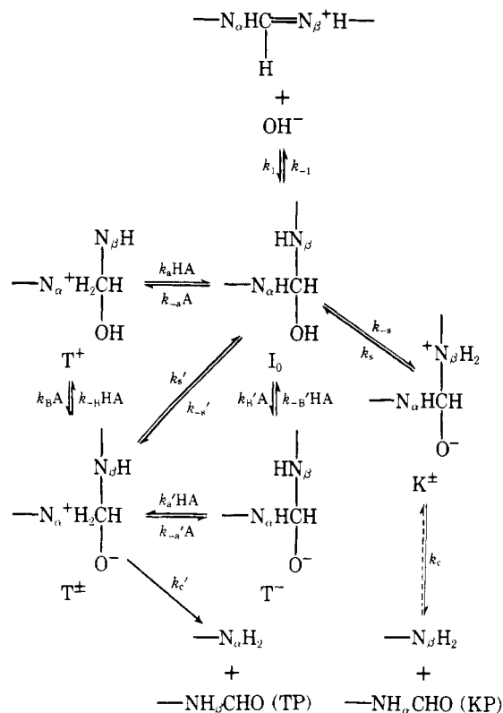
Scheme II
