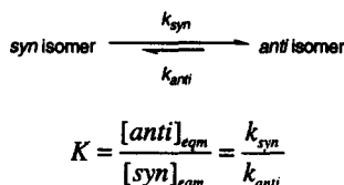
Scheme 2: Equilibration of atropisomeric diastereoisomers
