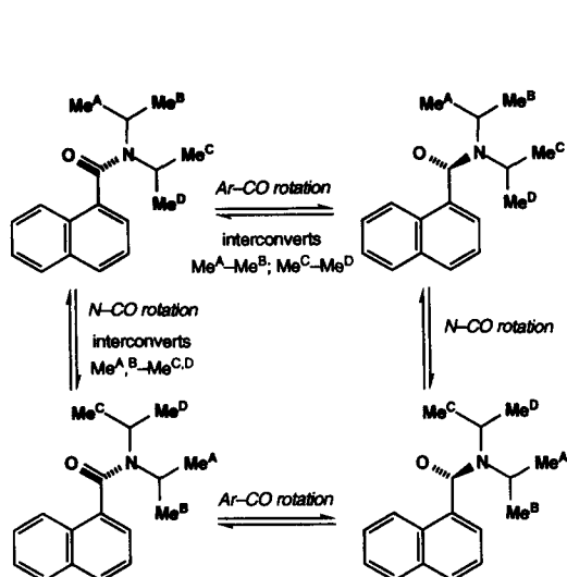
Scheme 1: Bond rotations in tertiary aromatic amide 4
