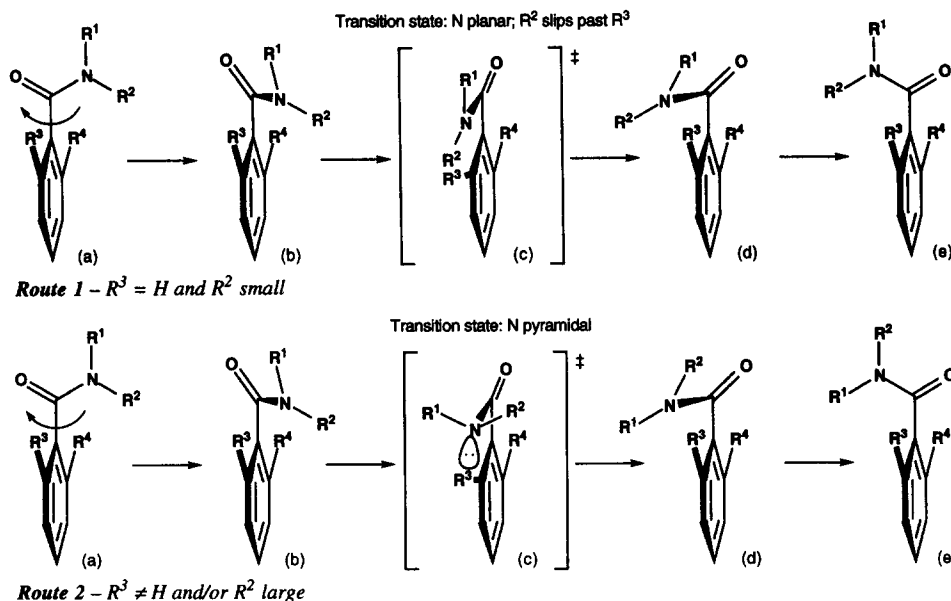
Scheme 3: Dynamics of Bond Rotation
