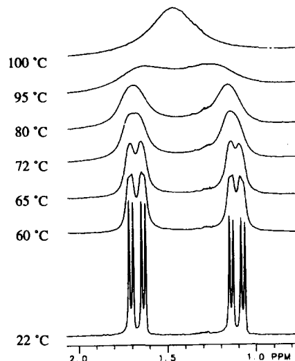
Figure 1: VT NMR experiments on amide 4
