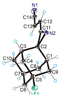
Figure 1. X-ray diffraction structure of 4f .
