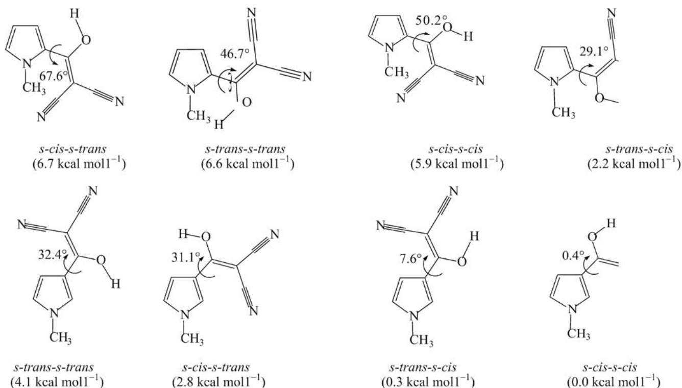
Fig. 1. Relative energies and deviation from planar structure of rotation conformations of 2- and 3-(1-hydroxy-2,2-dicyanoethenyl)-1-methylpyrroles IIh and IIIh optimized by method MP2/6-311G**.
