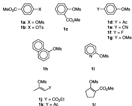
Fig. 1. Sulfonates 1 examined in Scheme 2.
