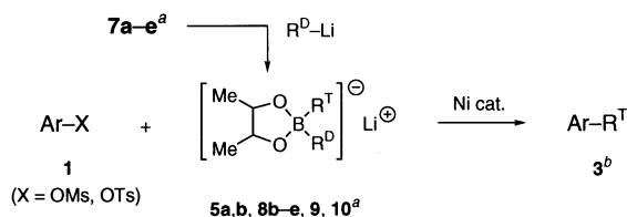
Scheme 2. Summary of the present study. a \text{R}^T and \text{R}^D in the boronates 7a–e and borates 5a,b, 8b–e, 9, 10 : see Eq. (2); b 3a : p\text{-MeO}_2\text{CC}_6\text{H}_4\text{-(2-furyl)} , 3b : p\text{-MeO}_2\text{CC}_6\text{H}_4\text{-C}_6\text{H}_5 . For other 3 , see Table 2.
