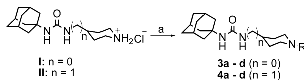
Scheme 2. Reagents and conditions: (a) bromoalkane, KI, DMF, K_2CO_3 , 50 °C, 12 h, 42–60%.
