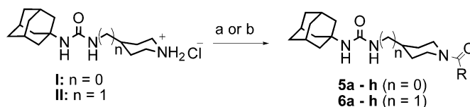
Scheme 3. Reagents and conditions: (a) \text{RCOCl} , TEA, DCM, 6 h, 20–73%; (b) \text{RCOOH} , TEA, DMAP, EDCI, dichloromethane, 0 °C to rt, 12 h, 75–99%.
