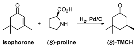
Figure 1. Proline directed asymmetric hydrogenation of isophorone to (S)-TMCH ((S)-3,3,5-trimethylcyclohexanone).
