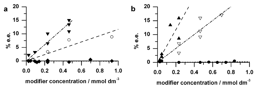
Figure 3. Dependence of TMCH ee on initial ligand concentration. Each data point corresponds to running the reaction up to a conversion of ~60%. (a) ▼, (S)-2-( tert -butylthiomethyl)pyrrolidine (4); ○, (S)-2-(methylthiomethyl)pyrrolidine (2); ◆, (S)-2-(phenylthiomethyl)pyrrolidine (6); (b) ▲, (S)-2-(adamantan-1-ylthiomethyl)-pyrrolidine (5); ▽, (S)-2-(iso-propylthiomethyl)pyrrolidine (3); ●, 1,2-bis((S)-pyrrolidin-2-ylmethyl)disulfane (1). A ligand concentration of 0.47 mmol dm -3 corresponds to 0.1 mol % ligand with respect to isophorone.
