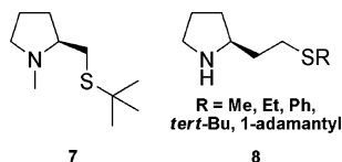
Figure 7. Modified sulfide ligands used in additional experiments ( S )-2-( tert -butylthiomethyl)-1-methylpyrrolidine ( 7 ) and ligands ( 8 ) containing an additional methylene unit between the pyrrolidine ring and the sulfide.
