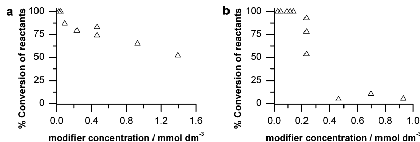
Figure 5. Dependence of activity (reactant conversion after a fixed time (168 h)) on ligand concentration. (a) ( S )-2-( tert -butylthiomethyl)pyrrolidine ( 4 ), (b) ( S )-2-(phenylthiomethyl)pyrrolidine ( 6 ).
