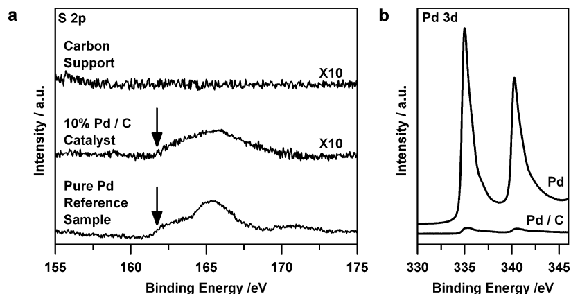
Figure 8. (a) Sulfur 2p XP spectra showing uptake of ( S )-2-( tert -butyl-thiomethyl)-pyrrolidine modifier ( 4 ) from methanol solution by (top to bottom) carbon support, 10 wt % Pd/C catalyst, and pure palladium reference sample. Samples were left in contact with ligand solution for 10 min. (b) Palladium 3d XP spectra for the fresh Pd/C catalyst and pure Pd reference.
