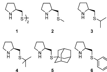
Figure 2. Sulfide ligands used 1,2-bis((S)-pyrrolidin-2-ylmethyl)disulfane (1), (S)-2-(methylthiomethyl)pyrrolidine (2), (S)-2-(iso-propylthiomethyl)pyrrolidine (3), (S)-2-( tert -butylthiomethyl)pyrrolidine (4), (S)-2-(adamantan-1-ylthiomethyl)pyrrolidine (5), and (S)-2-(phenylthiomethyl)pyrrolidine (6).
