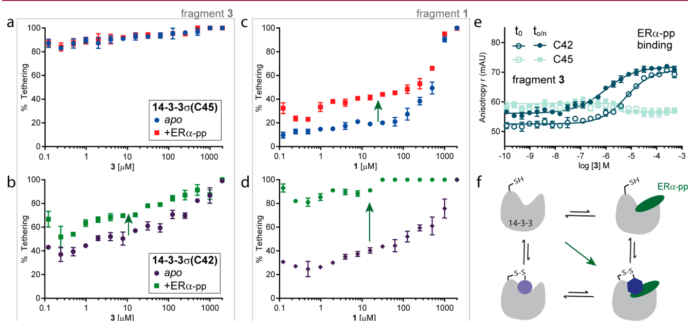
Figure 3. Analysis of cooperative binding to 14-3-3σ of tethered fragments with ERα-pp. Dose-response data of protein-fragment conjugate formation for 14-3-3σ C45 (a and c) or C42 (b and d), titrated with fragment 3 or 1, respectively, and analyzed by intact-protein mass spectrometry (MS). 100 nM 14-3-3σ, 200 nM ERα-pp, 100 μM fragment, 1 mM βME. (e) Fluorescence anisotropy dose-response curves for 14-3-3σ(C45 or C42) and fluorescein-labeled ERα-pp titrated with fragment 3. Data for time point 0 ( t 0 ) and at end point (after overnight incubation, t 0/n ) are displayed. (f) Schematic illustration of binding equilibria for ternary complex formation.
