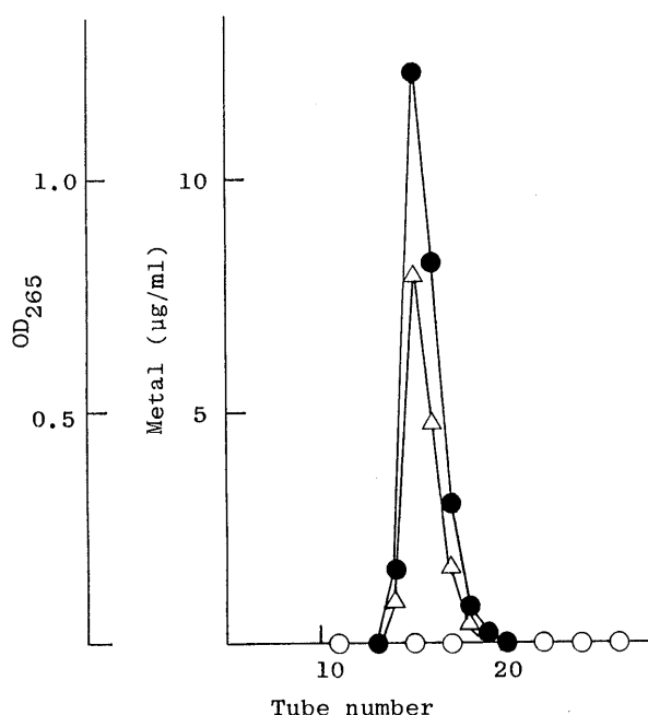
Fig. 5. Gel-Filtration of the Reaction Mixture of PC 5 and Cu + and Cd 2+ on a Sephadex G-10 Column
