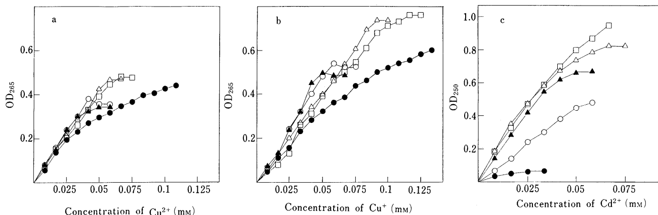
Fig. 4. Binding Properties of Peptides with Heavy Metals, a) with Cu 2+ , b) with Cu + , c) with Cd 2+
