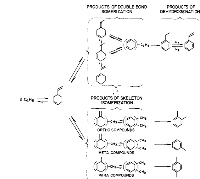
Figure 5. Scheme of formation of C_8 aromatics from butadiene via 4-vinylcyclohexene
