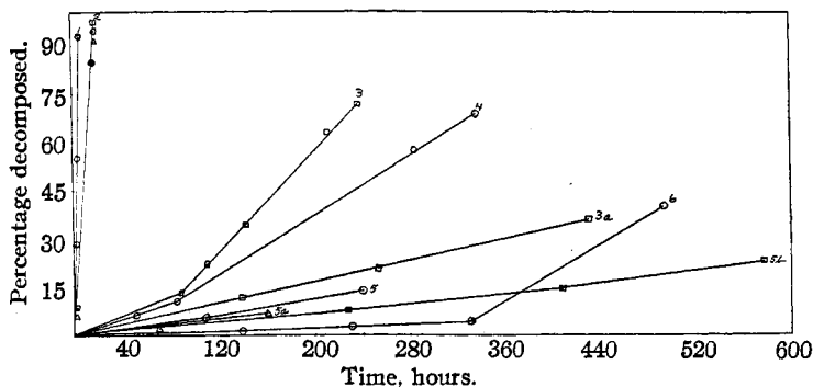
Fig. 1.—Rates of decomposition of ald-chlorimines at 30°. Curve 1, anisal- at 20–22°; o -methoxybenzal- gave approximately the same curve at 30°. Curve 2, points ○ and △, piperonal-; points □ and ⊗, o -nitrobenzal-. Curves 3 and 3a, o -chlorobenzal- (liq. at 30°). Curve 4, m -nitrobenzal-. Curves 5, 5a and 5b, p -chlorobenzal-. Curve 6, p -bromobenzal-.
