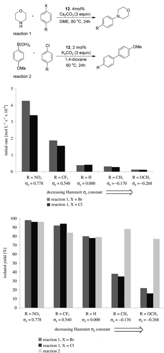
Figure 3. Top: Effect of p -substituted aryl halides (varying Hammett sigma constants ( \sigma_p )) on initial reaction rates for Pd-PEPPSI-IPr ( 12 )-catalyzed amination (reaction 1). Reaction rates were calculated from the linear portion ( t=0 to 240 min) of a product concentration versus time plot. Reactions were performed on a 2 mmol scale (aryl halide) with 3 mmol morpholine, 3 mmol \text{Cs}_2\text{CO}_3 and 4 mol % 12 in 2 mL 1,2-dimethoxyethane (DME) at 80 °C. Products were quantified by GC/MS analysis using undecane ( 100 \mu\text{L mmol}^{-1} of aryl halide) as a calibrated internal standard. Bottom: Effect of p -substituted aryl halides (varying Hammett sigma constants ( \sigma_p )) on isolated yields (24 h) for Pd-PEPPSI-IPr ( 12 )-catalyzed amination (reaction 1) and Suzuki–Miyaura reaction (reaction 2). Reactions were performed in duplicate and the average isolated yield is reported.
