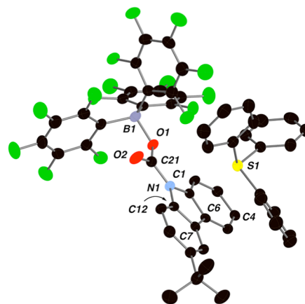
Figure 1. X-ray structure of 2-Ph 3 S (thermal ellipsoids drawn to 50% probability level). The tert -butyl group on C4 has been removed for clarity. Selected bond distances ( \text{\AA} ): B1–O1, 1.521(3) ; C21–O1, 1.310(3) ; C21–O2, 1.205(3) ; C21–N1, 1.393(3) . Selected non-bonded distances ( \text{\AA} ): S1–C1, 3.54 ; S1–C6, 3.49 ; S1–C7, 3.47 ; S1–C12, 3.47 ; S1–N1, 3.52 . Selected bond angle ( ^\circ ): B1–O1–C21, 121.9(2) .
