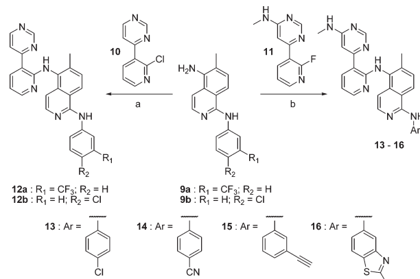
Scheme 2. Preparation of Aminoisoquinolines a
