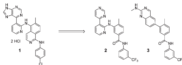
Figure 1. Structures of a potent, selective Raf inhibitor ( 1 ) and the screening leads 2 and 3 from which it was derived.
