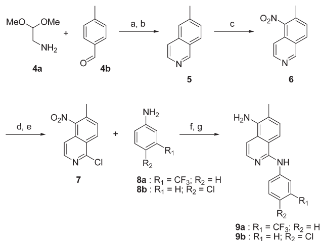
Scheme 1. Preparation of Aminoisoquinoline Intermediates a
