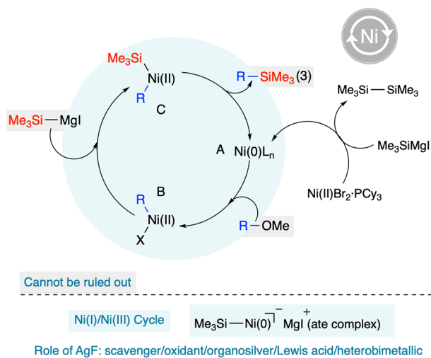
Scheme 4. Mechanistic Hypothesis
