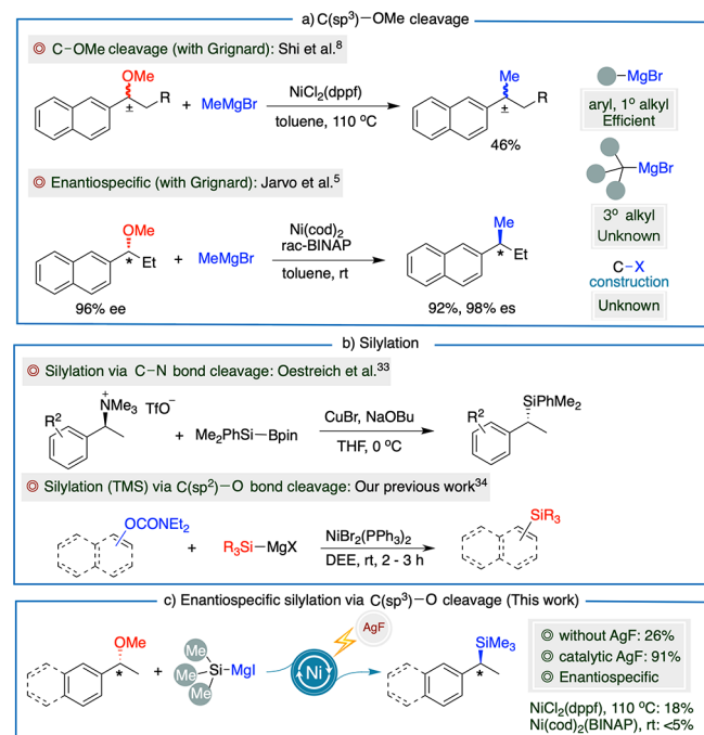
Scheme 1. Cross-Coupling Reactions via C–O Bond Cleavage
