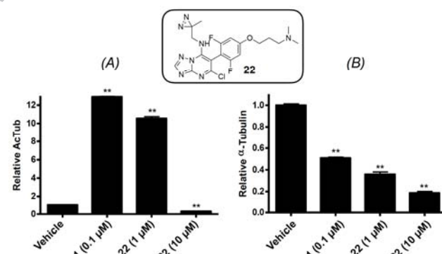
Figure 2. Relative changes of acetylated \alpha -tubulin (A) and total \alpha -tubulin (B) caused by 22 in HEK-293 cells after 4 h of incubation. **, p < 0.01 as determined by one-way ANOVA and Dunnett's post-hoc analysis.
