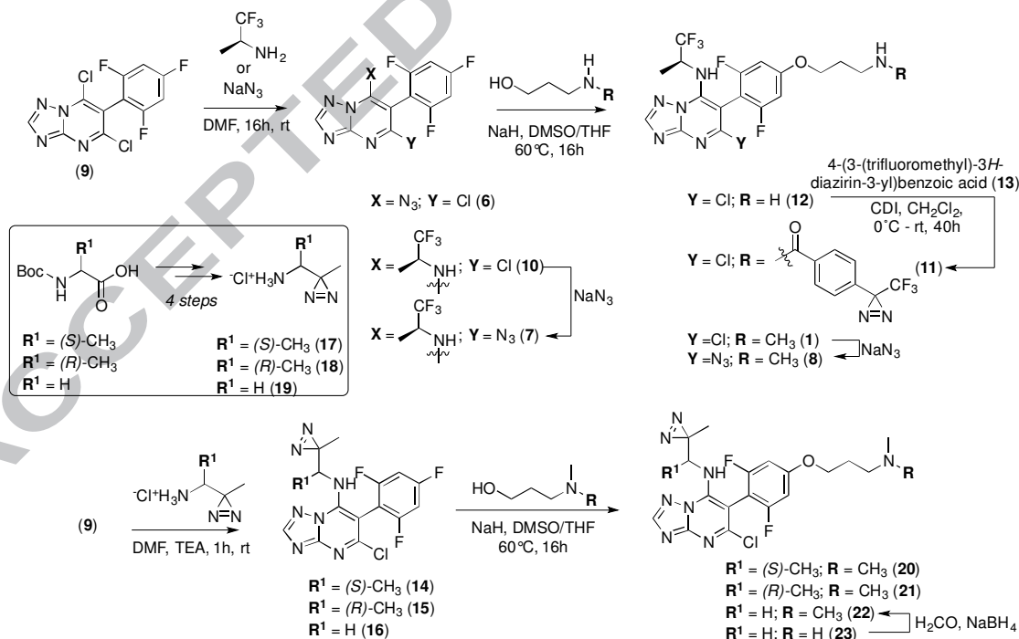
Scheme 1. Synthesis of triazolopyrimidine derivatives.
