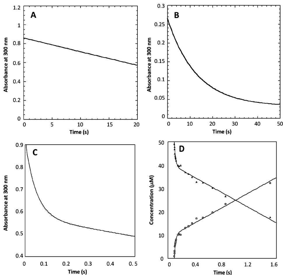
Figure 8. (A) Stopped-flow UV-vis trace of (20 \mu\text{M} ) E73D thioesterase-catalyzed hydrolysis of (80 \mu\text{M} ) 4-HB-CoA carried out under multiple turnover conditions and monitored at 300 nm ( \Delta\epsilon = 11.8 \text{ mM}^{-1} \text{ cm}^{-1} ). The trace was fitted with a linear equation. (B) Stopped-flow UV-vis trace of (40 \mu\text{M} ) E73D thioesterase-catalyzed hydrolysis of (20 \mu\text{M} ) 4-HB-CoA carried out under single turnover conditions and monitored at 300 nm. The trace was fitted with a single exponential equation. (C) Stopped-flow UV-vis trace of (30 \mu\text{M} ) T77A thioesterase-catalyzed hydrolysis of (100 \mu\text{M} ) 4-HB-CoA carried-out under multiple turnover conditions and monitored at 300 nm. The trace was fitted with a double exponential equation. (D) Time course for the multiple turnover reaction of 50 \mu\text{M} [^{14}\text{C}] 4-HB-CoA and 10 \mu\text{M} T77A thioesterase monitored using rapid quench/HPLC techniques. The data were fitted to a double exponential equation.
