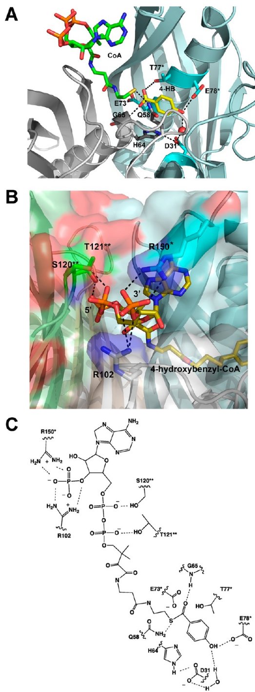
Figure 1. (A) The catalytic site of the Arthrobacter sp. strain SU 4-HB-CoA thioesterase bound with 4-HB and CoA (PDB accession 1Q4S). Only the AB dimer is shown. The nitrogen atoms are colored blue, the oxygen atoms are red and the sulfur atom yellow. The subunit A carbon atoms are colored red, whereas the subunit B carbon atoms are colored cyan. (B) The nucleotide binding site of the Arthrobacter sp. strain SU 4-HB-CoA thioesterase bound with 4-hydroxybenzyl-CoA (PDB accession 1Q4U). The ABCD tetramer is shown. The coloring scheme is the same as that stated in (A) but also includes the green-colored carbon atoms of subunit C and wheat colored-carbon atoms of subunit D. (C) The ChemDraw depiction of the proposed binding interactions between the thioesterase and the 4-HB-CoA substrate. The residues from subunits B and C are marked with * and **, respectively, and the hydrogen bonds are represented with dashed lines.
