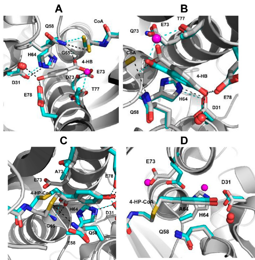
Figure 9. (A) Superposition of the X-ray structure of the wild-type thioesterase(4-HB)(CoA) complex with that of the E73D thioesterase(CoA) complex. (B) Superposition of the X-ray structure of the wild-type thioesterase(4-HB)(CoA) complex with that of the E73Q thioesterase(4-HB) complex. (C) Superposition of the X-ray structure of the wild-type thioesterase(4-HP-CoA) complex with that of the E73A/Q58E thioesterase(4-HP-CoA) complex. (D) Superposition of the X-ray structure of the wild-type thioesterase(4-HP-CoA) complex with that of the H64A thioesterase(4-HP-CoA) complex. Only the backbone of the wild-type thioesterase is shown. The nitrogen atoms are colored blue, the oxygen atoms red and the sulfur atom yellow. The carbon atoms are colored gray for the wild-type thioesterase and cyan for the mutant thioesterase.
