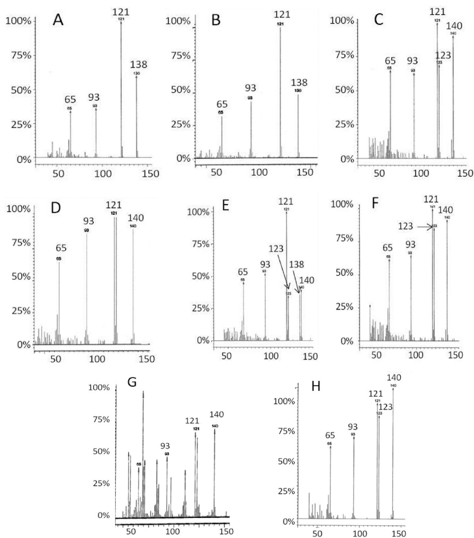
Figure 4. GC-MS spectra of 4-HB. The X and Y axes designate m/z units and relative intensity (%), respectively. (A) The 4-HB standard (parent ion m/z = 138 ). (B) The 4-HB produced by the (2.0 mM) wild-type thioesterase-catalyzed hydrolysis of 4-HB-CoA (0.2 mM) in natural isotopic abundance water. (C) The 4-HB produced by (2.0 mM) wild-type thioesterase-catalyzed hydrolysis of 4-HB-CoA (0.2 mM) in 97% \text{H}_2^{18}\text{O} . (D) The 4-HB produced by (2.0 mM) E73D thioesterase-catalyzed hydrolysis of 4-HB-CoA (0.2 mM) in 97% \text{H}_2^{18}\text{O} . (E) The 4-HB produced by (2.0 mM) T77A thioesterase-catalyzed 4-HB-CoA (0.2 mM) hydrolysis in 97% \text{H}_2^{18}\text{O} . (F) The 4-HB produced by (0.02 mM) T77A thioesterase-catalyzed hydrolysis of 4-HB-CoA (0.2 mM) in 97% \text{H}_2^{18}\text{O} . (G) The 4-HB produced by the (2.0 mM) T77S thioesterase-catalyzed hydrolysis of 4-HB-CoA (0.2 mM) in 97% \text{H}_2^{18}\text{O} . (H) The 4-HB produced by (2.0 mM) E73D/T77A thioesterase-catalyzed hydrolysis of 4-HB-CoA (0.2 mM) in 97% \text{H}_2^{18}\text{O} .
