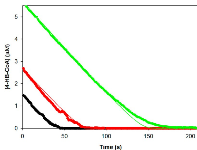
Figure 7. The time courses for the steady-state multiple-turnover reactions of 1.5 (green), 2.7 (red) or 5.7 (black) \mu\text{M} 4-HB-CoA catalyzed by 0.003 \mu\text{M} thioesterase in 50 mM \text{K}^+ HEPES (pH 7.5, 25 ^\circ\text{C} ). The 300 nm absorbance traces (dotted lines) are shown in the context of the calculated concentration of 4-HB-CoA ( \epsilon = 11.8 \text{ mM}^{-1} \text{ cm}^{-1} ) present in the reaction mixture (y-axis) as a function of reaction time (x-axis). The simulated curves (solid lines) were generated using the kinetic model shown in Scheme 3 and rate constants: k_1 = 192 \text{ }\mu\text{M}^{-1} \text{ s}^{-1} , k_{-1} = 30 \text{ s}^{-1} , k_2 = 44 \text{ s}^{-1} , k_{-2} = 14 \text{ s}^{-1} , k_3 = 36 \text{ s}^{-1} , k_{-3} = 0 \text{ s}^{-1} , k_4 = 129 \text{ s}^{-1} , k_{-4} = 5 \text{ }\mu\text{M}^{-1} \text{ s}^{-1} , k_5 = 368 \text{ }\mu\text{M}^{-1} \text{ s}^{-1} and k_{-5} = 5 \text{ }\mu\text{M}^{-1} \text{ s}^{-1} .
