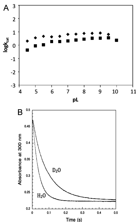
Figure 3. (A) A plot of \log k_{\text{cat}} vs reaction solution pL measured for wild-type thioesterase catalyzed hydrolysis of 4-HB-CoA in buffered H 2 O (◆) or buffered D 2 O (■). (B) A stopped-flow UV-vis absorbance trace (300 nm) of (40 μM) wild-type thioesterase-catalyzed hydrolysis of (20 μM) 4-HB-CoA carried out at 25 °C in buffered H 2 O or buffered D 2 O (pL = 7.5). The data were fitted with a single exponential equation.
