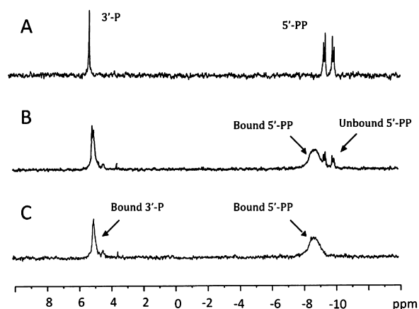
Figure 10. 31 P NMR spectrum of (A) 1 mM 4-HP-CoA, (B) 1.5 mM 4-HP-CoA and 1 mM wild-type thioesterase, and (C) 1 mM 4-HP-CoA and 1 mM wild-type thioesterase. See Materials and Methods for details.
