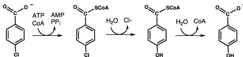
Scheme 1. Three Chemical Steps of the 4-Chlorobenzoate Dehalogenation Pathway Catalyzed by 4-Chlorobenzoate: CoA Ligase, 4-Chlorobenzoyl-CoA Dehalogenase and 4-Hydroxybenzoyl-CoA Thioesterase, Respectively
