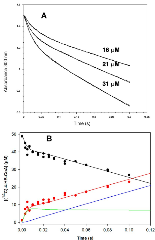
Figure 2. (A) Stopped-flow UV-vis absorbance traces of (16, 21, and 31 \mu\text{M} ) wild-type thioesterase-catalyzed hydrolysis of (112 \mu\text{M} ) 4-HB-CoA carried out under multiple turnover conditions and monitored at 300 nm ( \Delta\epsilon = 11.8 \text{ mM}^{-1} \text{ cm}^{-1} ). The traces were fitted using a double exponential equation. (B) The time course for the multiple turnover reaction of 50 \mu\text{M} [ ^{14}\text{C} ]4-HB-CoA and 10 \mu\text{M} thioesterase monitored using rapid quench/HPLC techniques. The curves were simulated using the kinetic model shown in Scheme 3 and the microscopic rate constants k_1 = 172 \mu\text{M}^{-1} \text{ s}^{-1} , k_{-1} = 30 \text{ s}^{-1} , k_2 = 264 \text{ s}^{-1} , k_{-2} = 9 \text{ s}^{-1} , k_3 = 25 \text{ s}^{-1} , k_{-3} = 0 \text{ s}^{-1} , k_4 = 129 \text{ s}^{-1} , k_{-4} = 5 \mu\text{M}^{-1} \text{ s}^{-1} , k_5 = 368 \mu\text{M}^{-1} \text{ s}^{-1} and k_{-5} = 5 \mu\text{M}^{-1} \text{ s}^{-1} . The simulated curve-coloring scheme is as follows: E-I(CoA) + E(4-HB)(CoA) + E(4-HB) + 4-HB (red); E(4-HB-CoA) + 4-HB-CoA (black); E-I(CoA) (green); E(4-HB)(CoA) + 4-HB (blue).
