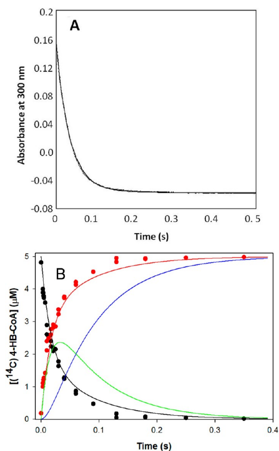
Figure 6. (A) Stopped-flow UV-vis absorbance trace of (40 \mu\text{M} ) wild-type thioesterase-catalyzed hydrolysis of 4-HB-CoA (20 \mu\text{M} ) carried out under single turnover conditions and monitored at 300 nm ( \Delta\epsilon = 11.8 \text{ mM}^{-1} \text{ cm}^{-1} ). (B) Time course for the single turnover reaction of 5 \mu\text{M} [ ^{14}\text{C} ]4-HB-CoA and 50 \mu\text{M} thioesterase monitored using rapid quench/HPLC techniques. The data were fitted to a double exponential equation. The curves were simulated using the kinetic model shown in Scheme 3 and the microscopic rate constants k_1 = 194 \text{ }\mu\text{M}^{-1} \text{ s}^{-1} , k_{-1} = 30 \text{ s}^{-1} , k_2 = 44 \text{ s}^{-1} , k_{-2} = 14 \text{ s}^{-1} , k_3 = 17 \text{ s}^{-1} , k_{-3} = 0 \text{ s}^{-1} , k_4 = 129 \text{ s}^{-1} , k_{-4} = 5 \text{ }\mu\text{M}^{-1} \text{ s}^{-1} , k_5 = 368 \text{ }\mu\text{M}^{-1} \text{ s}^{-1} , and k_{-5} = 5 \text{ }\mu\text{M}^{-1} \text{ s}^{-1} . The simulated curve-coloring scheme is as follows: E-I(CoA) + E(4-HB)(CoA) + E(4-HB) + 4-HB (red); E(4-HB-CoA) + 4-HB-CoA (black); E-I(CoA) (green); E(4-HB)(CoA) + E(4-HB) + 4-HB (blue).
