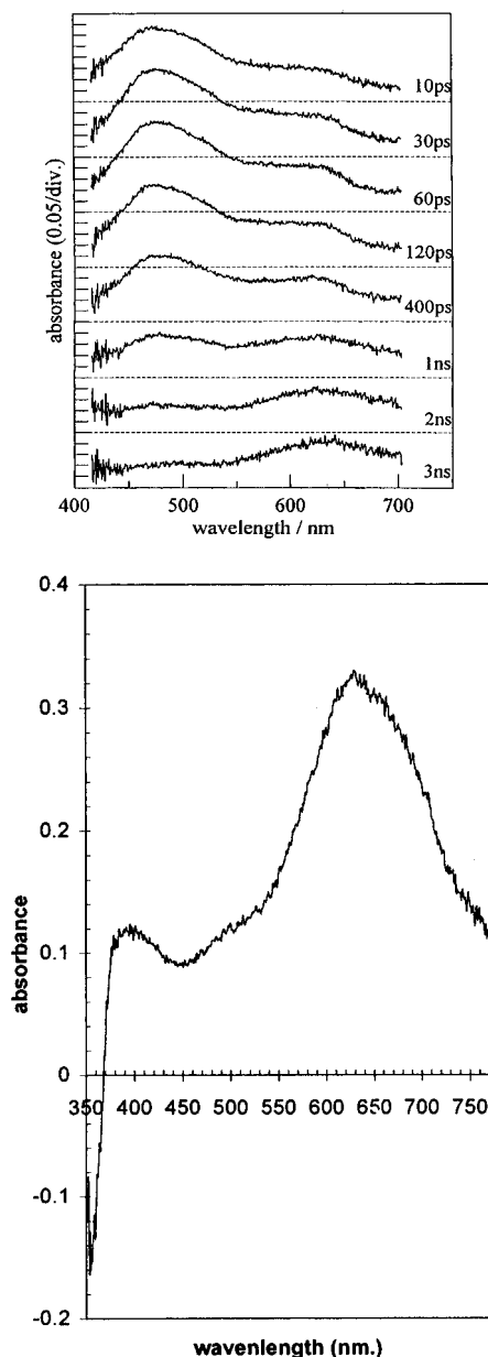
Figure 6. Transient absorption spectra of pEFTP iso-octane: (a, top) picosecond transient absorption spectra from 10 ps to 3 ns after excitation, and (b, bottom) nanosecond transient absorption spectra 100 ns after excitation.
