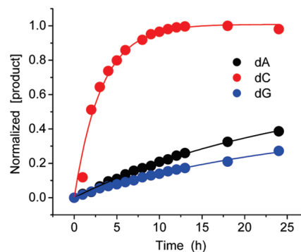
Figure 2. 1,4-Butanediol adduct formation with nucleosides as a function of time.
