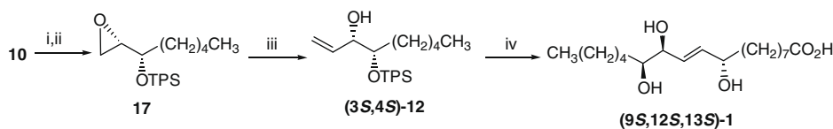
Scheme 2. Reagents and conditions: (i) TMSCl/EtOAc/–20 °C/20 min; MsCl/Et 3 N/–20 °C/30 min; 2 N aqueous HCl/25 °C/40 min (78%); (ii) NaH/THF/0–25 °C/3 h (89%); (iii) Me 3 Si/BuLi/THF/–25 °C/1 h then 25 °C/6 h (84%); (iv) As in Scheme 1.
