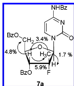
Figure 2. ^1\text{H} NMR NOE correlations of compound 7a .
