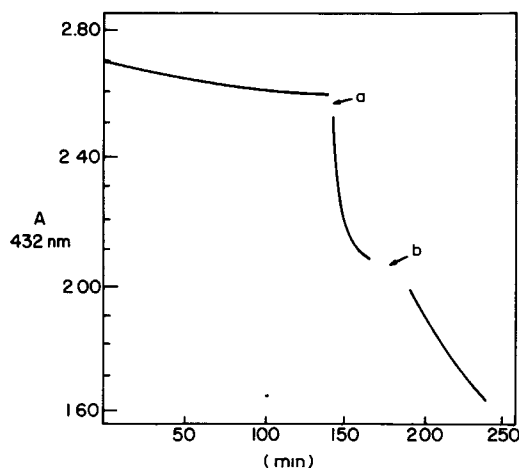
Fig. 2 Reaction of hexamethylditin and N -chlorosuccinimide in chloroform at 25°, in presence of 0.3 mole % galvinoxyl, degassed. At (a) Nitrogen containing 0.2% O 2 added (b) Nitrogen containing 1.0 mole % O 2 added
