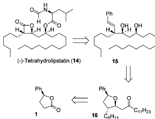
FIGURE 3. Retrosynthetic analysis for (–)-tetrahydrolipstatin.
