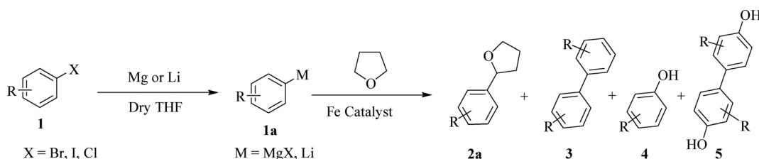
Scheme 1 Iron oxide catalyzed cross-coupling reaction of organometallic species with THF via activation of \alpha\text{-C}(\text{sp}^3)\text{--H} .
