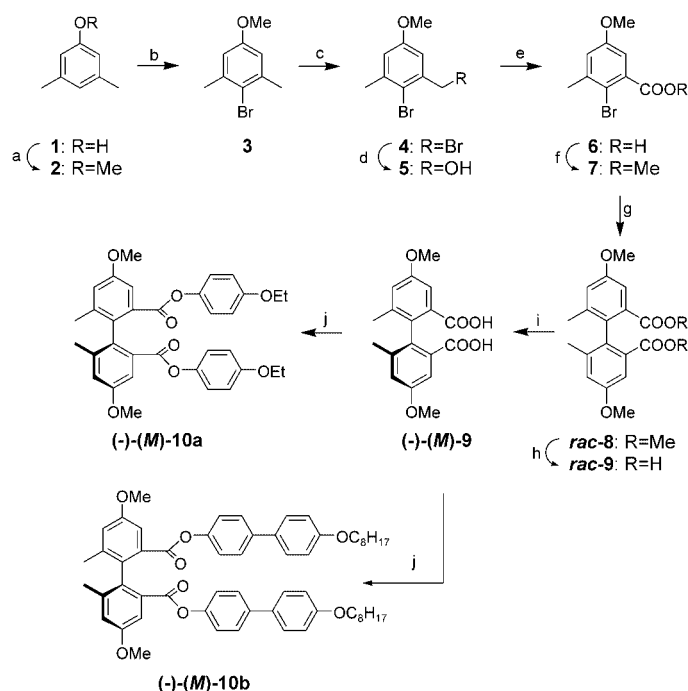
Scheme 1. Reaction conditions: a) KOH, MeOH, Me 2 SO 4 (84%); b) CCl 4 , Br 2 , -5°C (85%); c) CCl 4 , NBS;AIBN; reflux (92%); d) dioxane water, CaCO 3 , reflux (95%); e) acetone, KMnO 4 , reflux (85%); f) SOCl 2 , MeOH (93%); g) Cu, DMF, reflux (92%); h) NaOH, water, reflux (97%); i) brucine, MeOH, acetone, HCl (38%); j) THF, CH 3 SO 2 . Cl, Et 3 N, -25°C; 10a : p -ethoxyphenol (63%), 10b : 4'-octyloxy(1,1'-biphenyl)-4-ol (59%).
