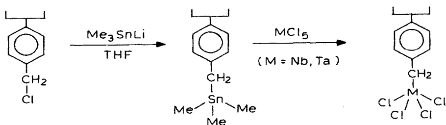
SCHEME 2. Preparation of Polymer-Attached (\eta^1\text{-PhCH}_2)\text{MCl}_4 ( M = \text{Nb} and \text{Ta} )
