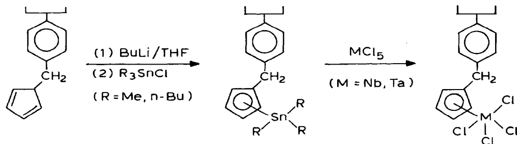
SCHEME 1. Preparation of polymer-attached \text{CpMCl}_4 ( M = \text{Nb} , \text{Ta} ).
