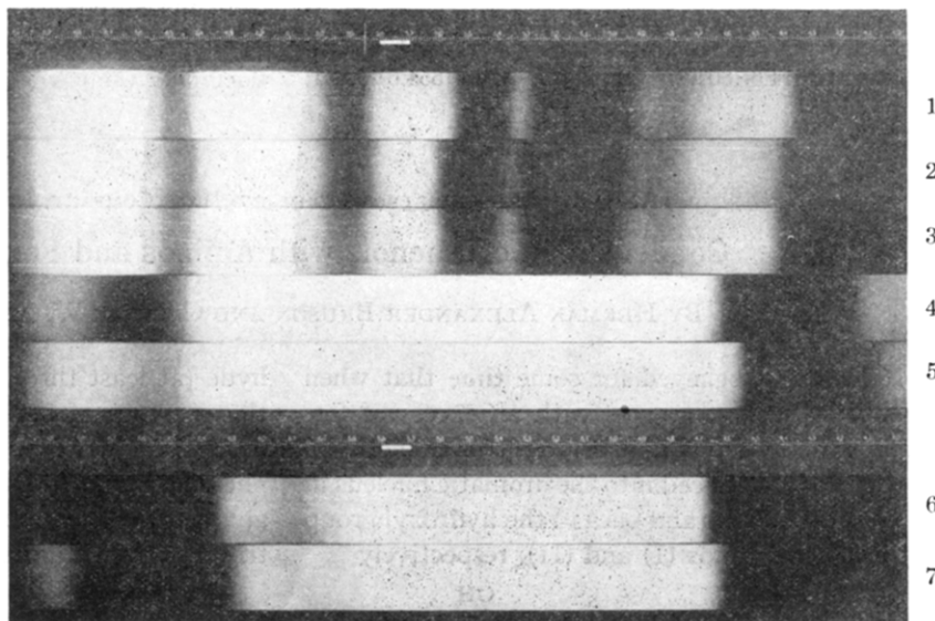
Fig. 3.—Absorption spectra of \alpha,\beta,\gamma,\delta -tetraphenylporphyrin: 1, in ether, 0.25 m ; 2, in chloroform, 0.25 m ; 3, in pyridine, 0.25 m ; 4, in chloroform containing hydrogen chloride, 0.12 m ; 5, in glacial acetic acid, 0.12 m ; 6, same as 4, but 0.25 m ; 7, same as 5, but 0.25 m .
