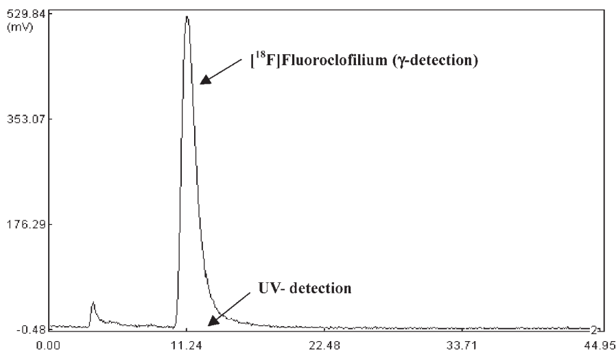
Figure 1. HPLC analysis of the purified [ ^{18}\text{F} ]Fluoroclofilium (2). UV (277 nm) and \gamma -detection (511 keV) profiles were recorded simultaneously. HPLC was performed on a reverse-phase column (Nova-Pak \text{C}_{18} , 3.9 \times 300 mm, 4\mu\text{m} . Eluent: MeOH/0.05 M \text{K}_2\text{HPO}_4 with 10% MeOH 60/40 at a flow rate of 1 ml/min)
