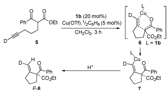
Scheme 2. Proposed Mechanistic Pathway via a Copper Enolate
