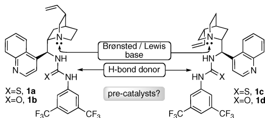
Figure 1. Pseudoenantiomeric cinchona-derived potential precatalysts to Brønsted base/Lewis acid cooperative catalysts.
