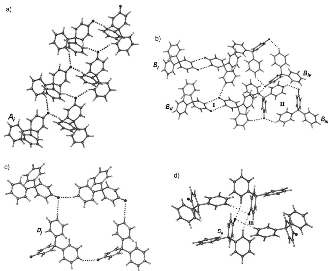
Figure 1. a) Helices of C–H \cdots O hydrogen bonds (2.55 Å, 163.6°; 2.60 Å, 129.9°) between 2 1 related molecules in form A [conformer A i , graph set C(8)]. b) Centrosymmetric C–H \cdots O synthon I between B i , B ii molecules of R 2 2 (8) pattern (2.33 Å, 169.2°; 2.49 Å, 123.5°) and synthon II between B iii , B iv molecules of R 2 2 (20) pattern (2.64 Å, 138.0°; 2.74 Å, 121.6°) in form B . The crystal structure of form C is similar to B . Twelve symmetry independent molecules (C i –C xii ) engage in similar synthons instead of four molecules in B . c) C–H \cdots O interactions of graph set R 4 3 (32) between translation and screw-axis-related D i molecules (2.36 Å, 137.9°; 2.54 Å, 166.9°) in form D . d) Centrosymmetric C–H \cdots O synthon III between D ii molecules [R 2 2 (16) pattern] and C–H \cdots O interaction (2.57 Å, 144.5°; 2.47 Å, 165.1°). Neutron-normalized distances are quoted. Note that different C–H donors participate in C–H \cdots O interactions in different crystal forms. Cyclic C–H \cdots O synthons I–III are labeled.
