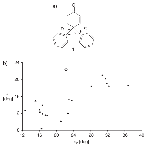
Figure 7. a) Conformations of diphenylquinone 1 defined by torsion angles \tau_1 and \tau_2 about the C quinone -C phenyl single bonds. b) Nineteen crystallographically independent conformations of 1 lie along the diagonal. All 19 conformers converge to the gas-phase rotamer ( \tau_1 = \tau_2 = 22.3^\circ ) after energy minimization. A = ●, B = ■, C = ▲, D = ◆, and gas phase = ⊗.
