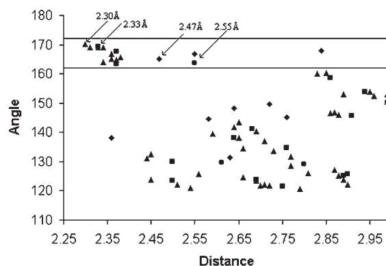
Figure 2. H \cdots O distance (2.2–3.0 Å) versus C–H \cdots O angle (120–180°) scatter plot of interactions in tetramorphs A–D. A = ● (Z' = 1), B = ■ (Z' = 4), C = ▲ (Z' = 12), D = ◆ (Z' = 2). The shortest H \cdots O distance (marked with an arrow in the linear band) is inversely related to Z' (the number of symmetry-independent conformations).
